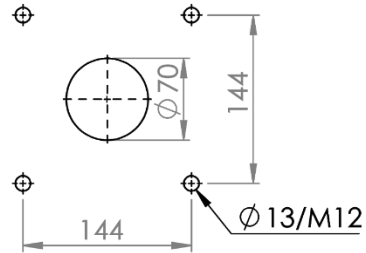
Mounting Cut-Out
